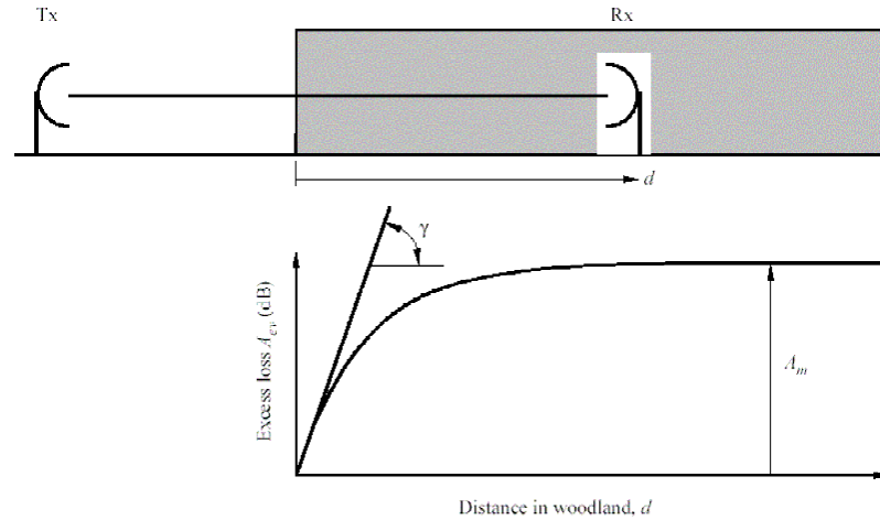
Figure 4.2: Representative radio path in woodland (ITU-R Rec. P.833)
