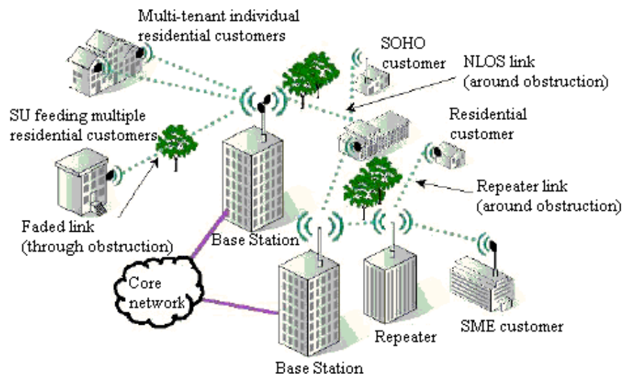
Figure 3.2: Example of a point-to-multipoint network deployment (ETSI TR 101 856)
