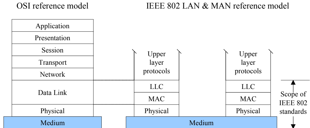
Figure 3.1: IEEE 802 LAN & MAN reference model (Adapted from: IEEE Std 802-2001)
