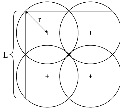
Figure 6.5: Four cells covering a square-shaped area
