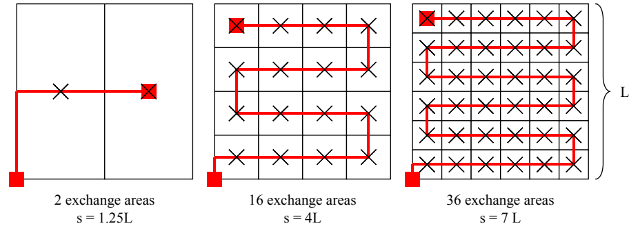
Figure 6.6: Fiber backbone network dimensioning
