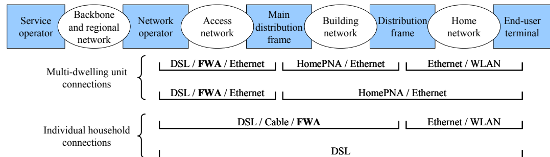
Figure 2.2: Positioning of different technologies in the broadband network structure
