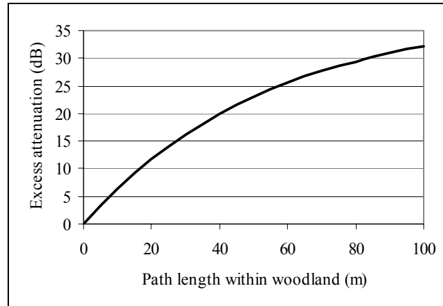
Figure 4.3: Attenuation in vegetation as a function of distance for a 3.5 GHz signal
