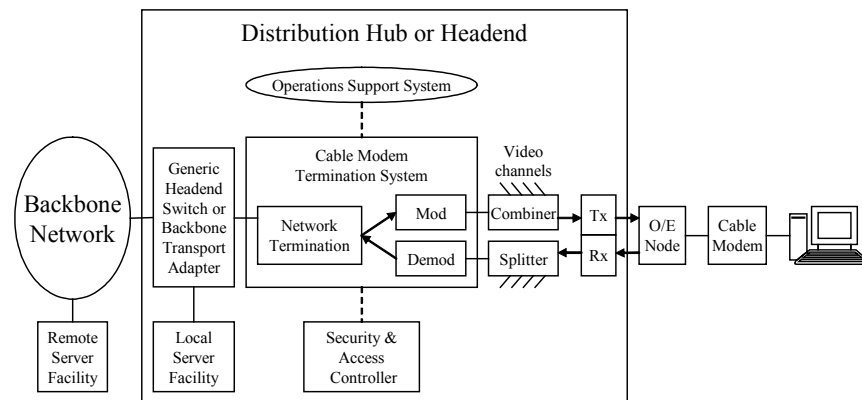
Figure 2.6: Data-over-cable network architecture (adapted from CableLabs 2002)
