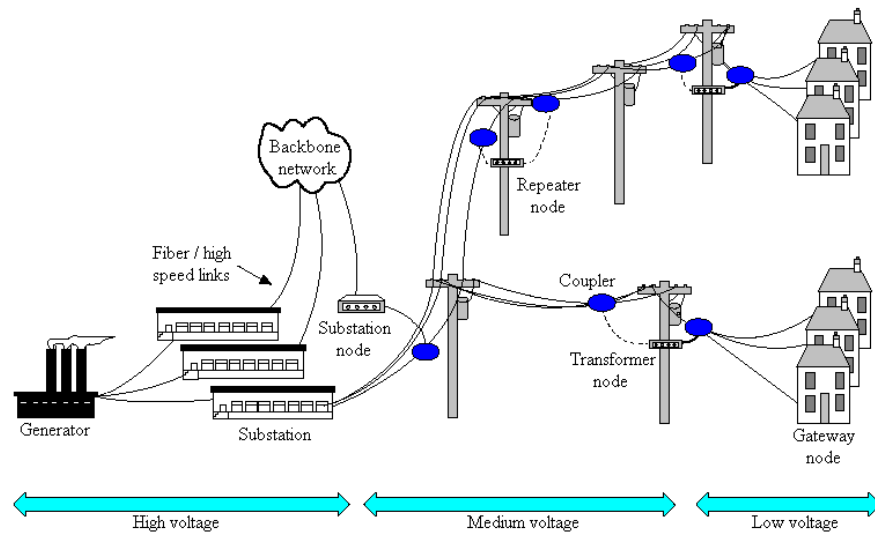
Figure 2.7: PLC system architecture (redrawn from Jee et al. 2003)
