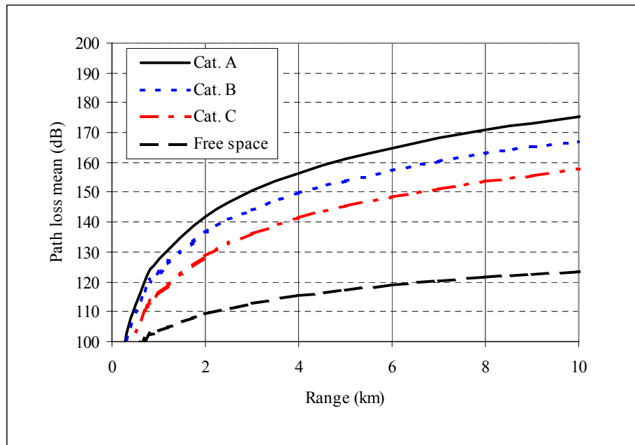
Figure 4.1: Exemplary path loss curves calculated using the 802.16 channel models and the Friis' free space path loss model
