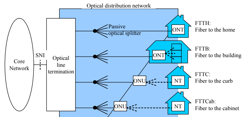
Figure 2.4: The fiber-to-the-x (FTTx) concept (adapted from Maeda et al. 2001)
