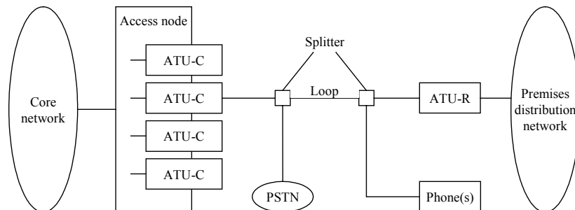
Figure 2.5: ADSL system reference model (adapted from ADSL Forum TR-001 1997)
