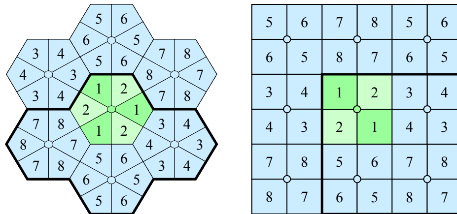
Figure 4.4: Possible frequency reuse patterns using 8 channels
